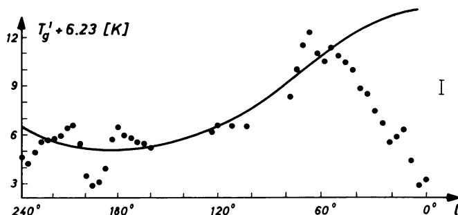
Figure 1. The T'_g distribution for b=38^\circ . The dots are values of T'_g+6.23 computed from data at 38 and 408 MHz for \beta_c=2.5 . The curve corresponds to the best-fit spheroid (19, 18.75 kpc) matched to the dots for \ell>40^\circ .
